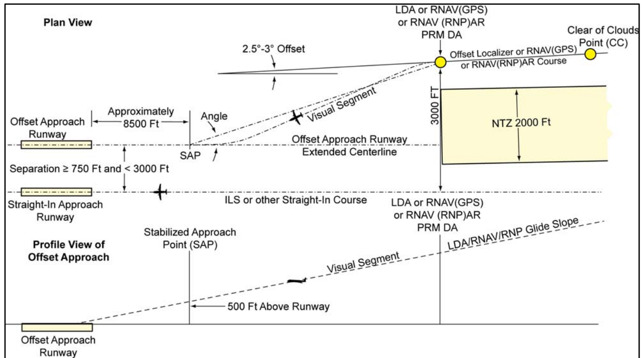
FIG 5-4-23 SOIA Approach Geometry
