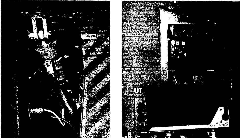
PHOTO 4 AFT STRUT ASSEMBLY OF STAN AND STOW WEIGHT AND BALANCE SYSTEMS .
