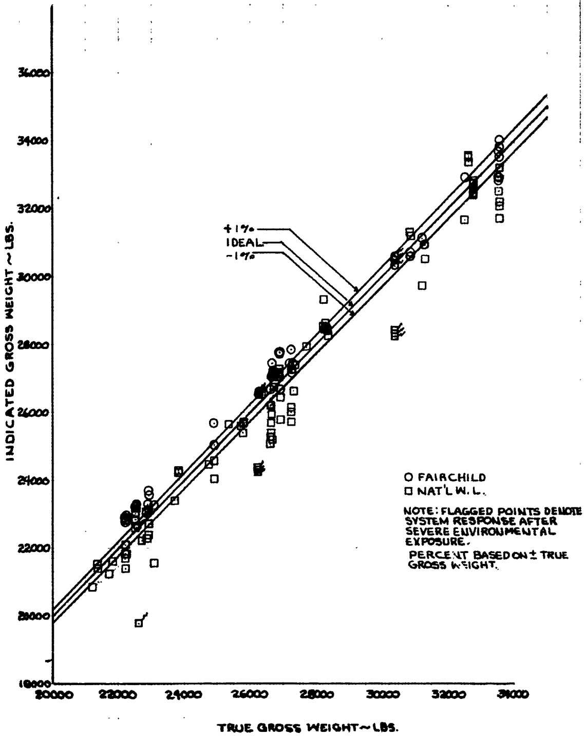
FIGURE NO. 2 VARIATION OF INDICATED GROSS WEIGHT CH-47A S/N 468106 STATIC CONDITION
