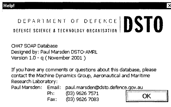
Figure 6. Help screen
