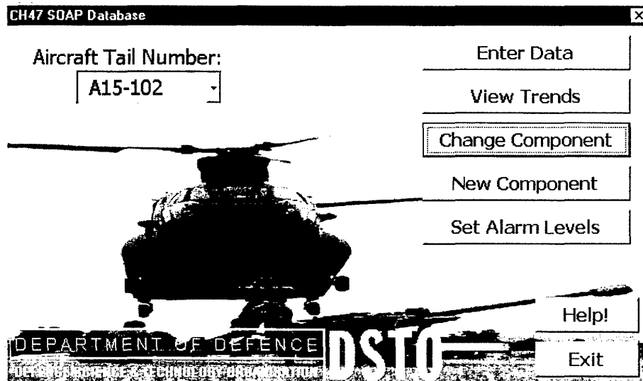
Figure 1. Introduction screen
