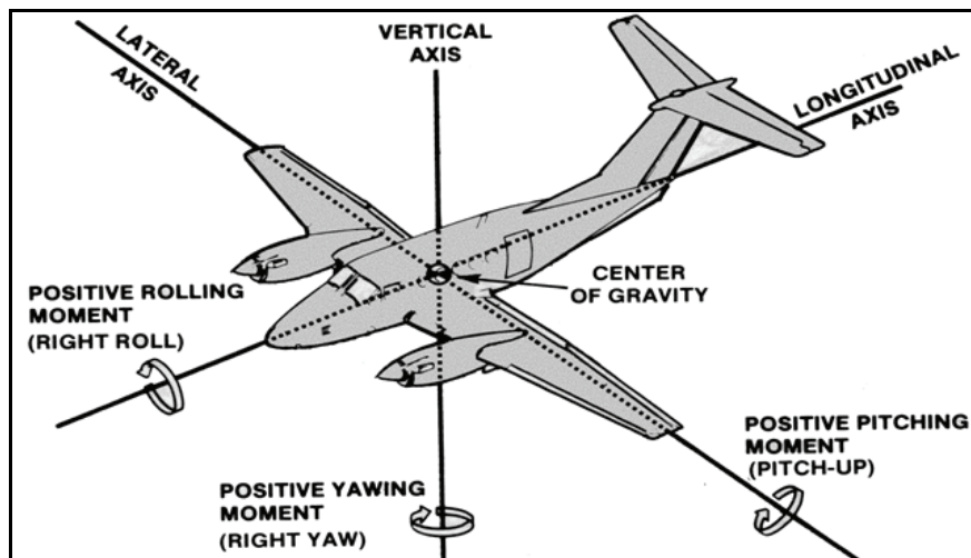
Figure 7-1. Stability nomenclature
