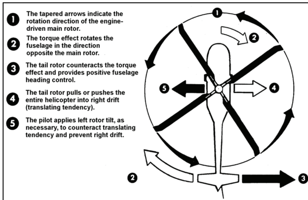
Figure 1-51. Translating tendency
