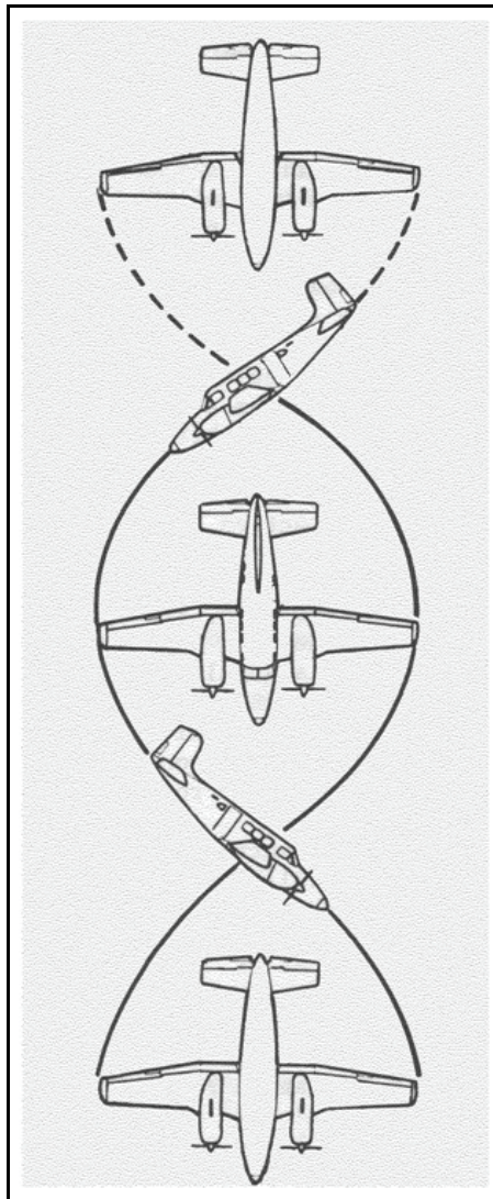
Figure 7-36. Spins
