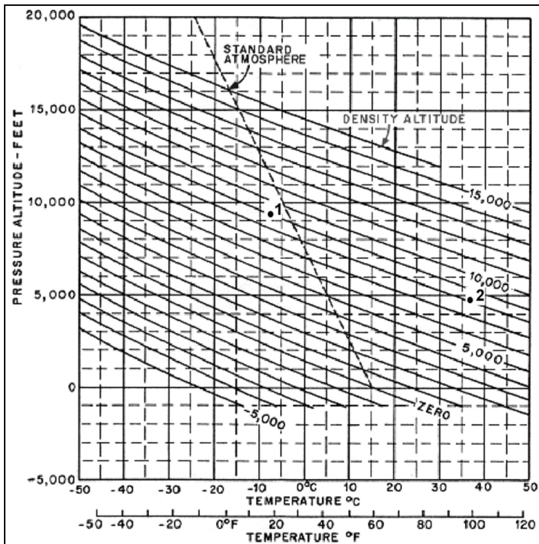
Figure 1-72. Density altitude computation
