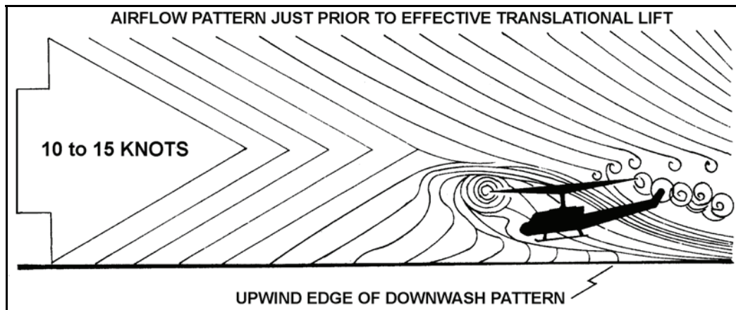
Figure 1-58. Translational lift (10 to 15 knots)
