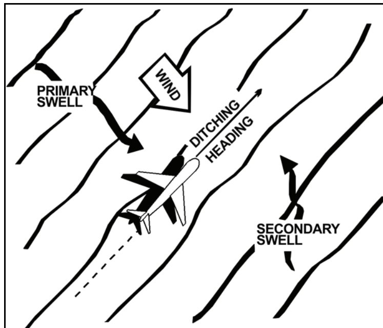
Figure 8-7. Single swell
