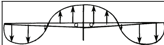
Figure 1-74. Induced flow velocity before vortex ring state
