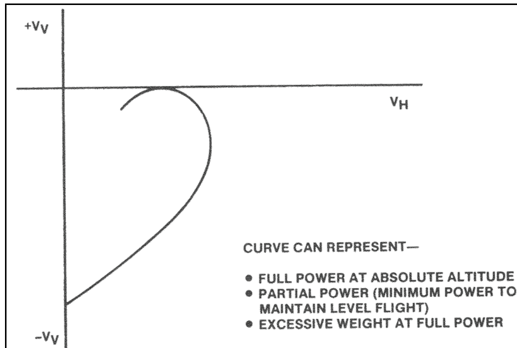
Figure 7-41. Polar curve
