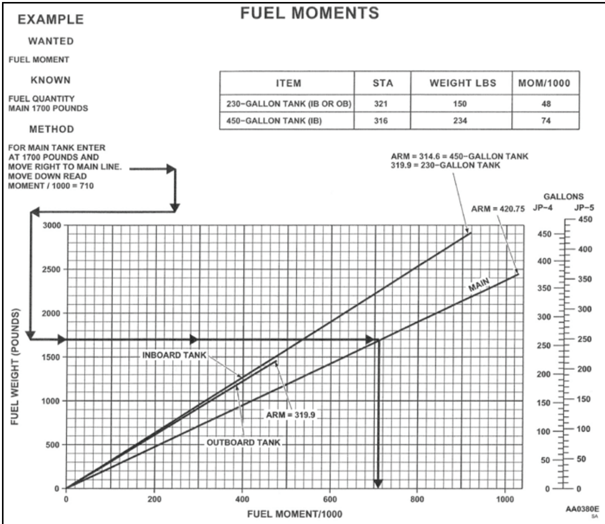
Figure 2-4. Fuel moments
