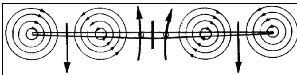
Figure 1-75. Vortex ring state
