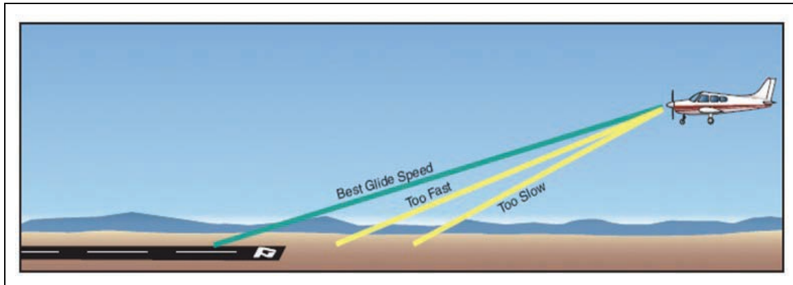
Figure 7-44. Best glide speed
