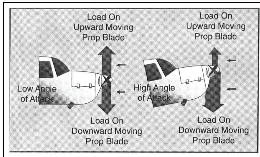
Figure 7-22. Asymmetric loading (propeller-factor)
