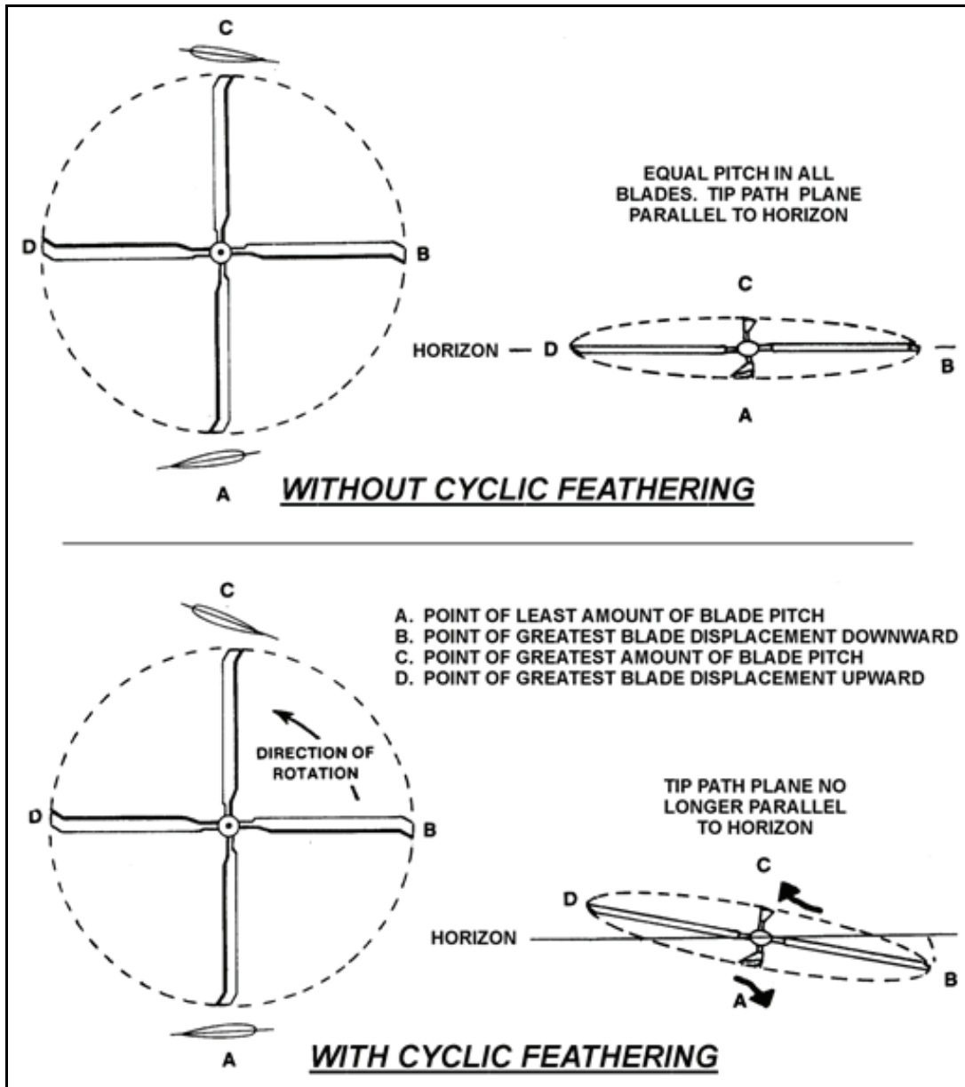
Figure 1-31. Cyclic feathering
