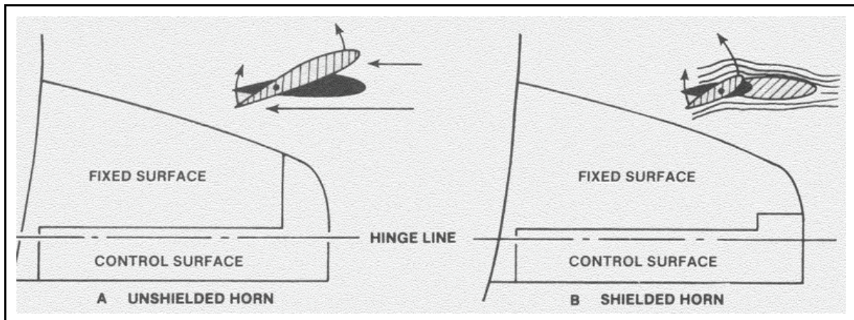
Figure 7-53. Aerodynamic balancing using horns
