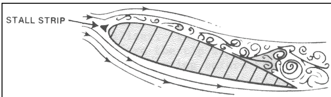
Figure 7-34. Stall strip
