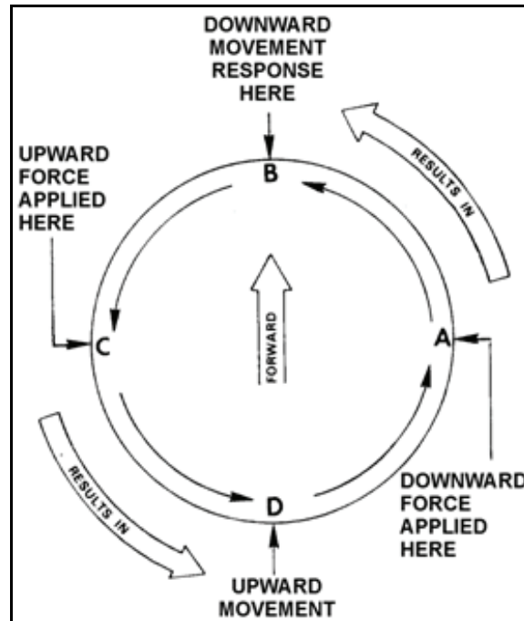
Figure 1-25. Gyroscopic precession
