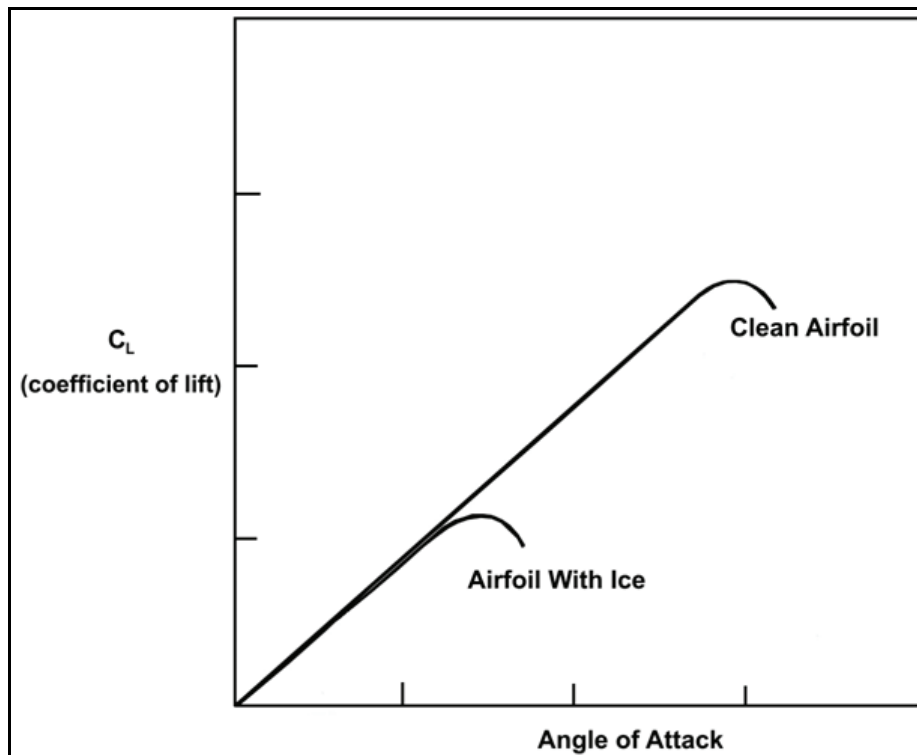
Figure 8-1. Lift curve
