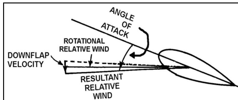
Figure 1-55. Flapping (retreating blade, 9-o'clock position)
