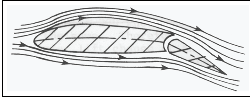
Figure 7-47. Using flaps to increase camber
