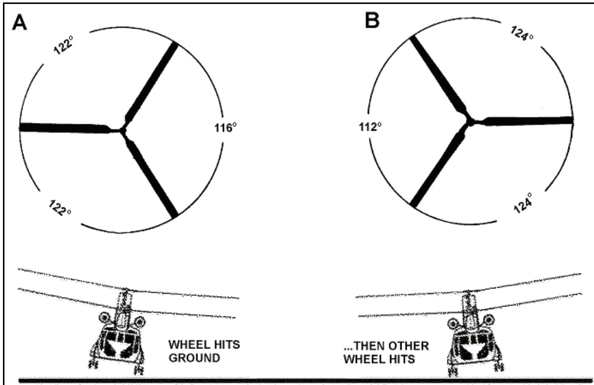
Figure 1-82. Ground resonance
