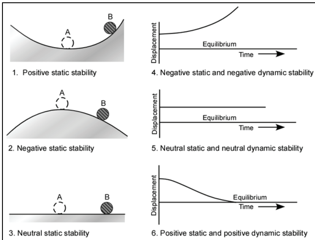
Figure 7-2. Nonoscillatory motion
