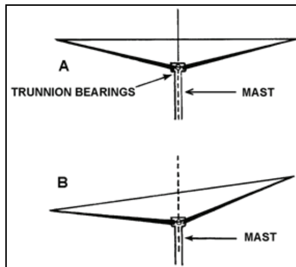
Figure 1-35. Semirigid rotor system
