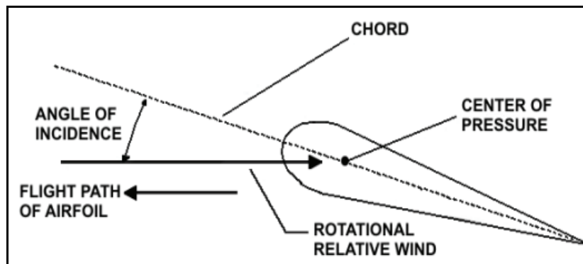
Figure 1-12. Rotational relative wind
