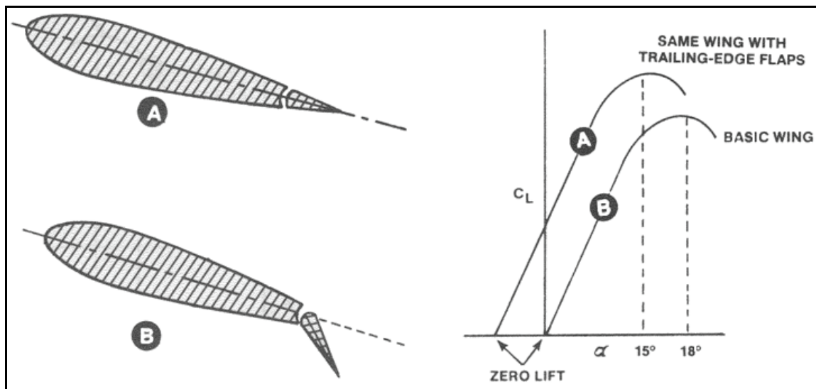
Figure 7-23. Increasing camber with trailing-edge flap
