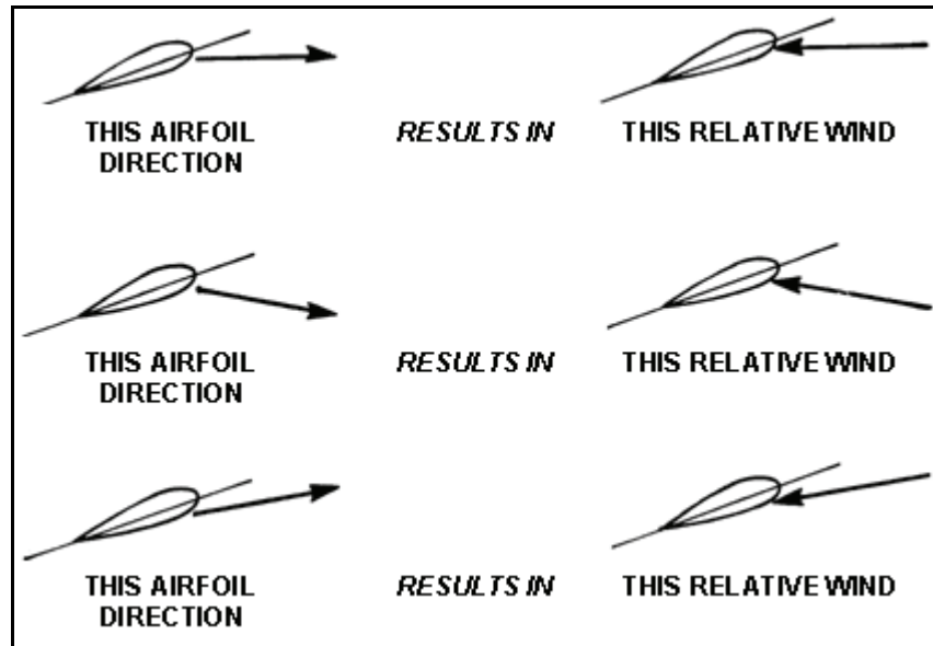
Figure 1-11. Relative wind
