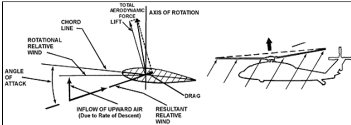
Figure 1-66. Force vectors in autorotative steady-state descent
