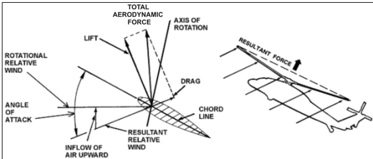
Figure 1-67. Autorotative deceleration
